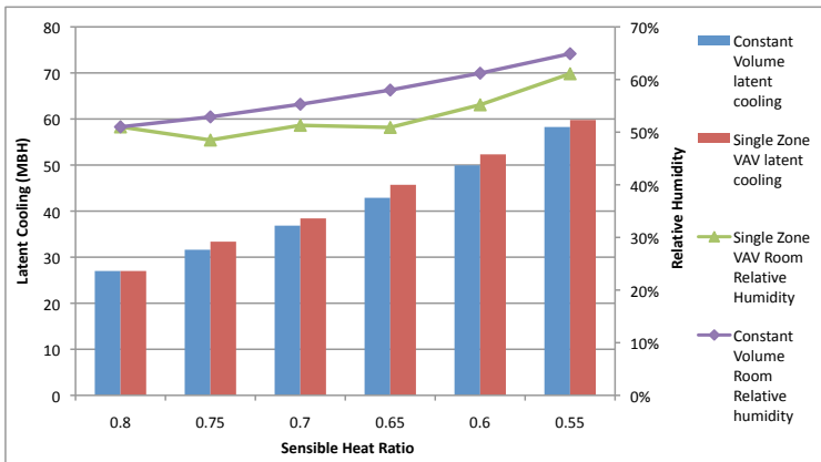
Figure 19: Latent Cooling and Relative Humidity (Increased Latent Load) versus Sensible Heat Ratio
